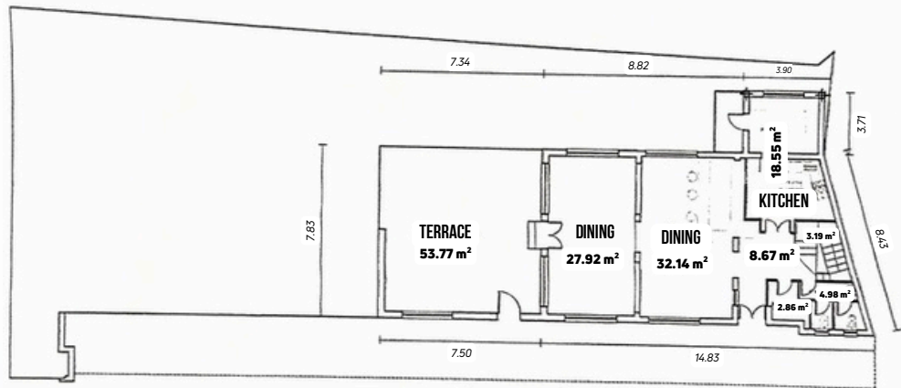
TOP FLOOR (KITCHEN, DINING, TERRACE)
