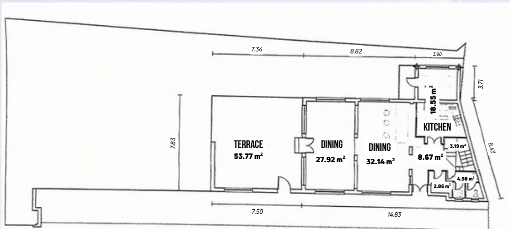
TOP FLOOR (KITCHEN, DINING, TERRACE)
